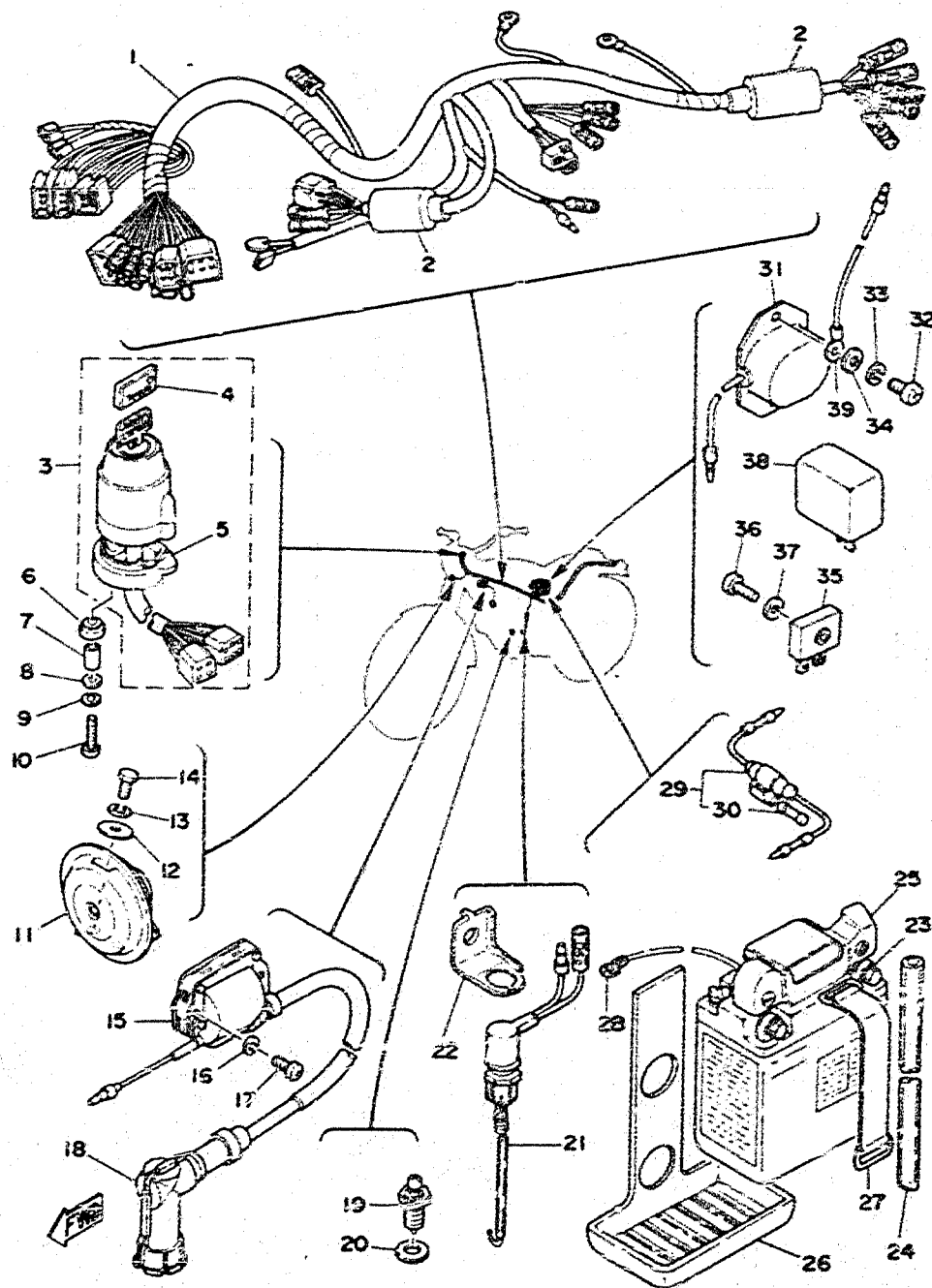
Fig. 40 ELECTRICAL
