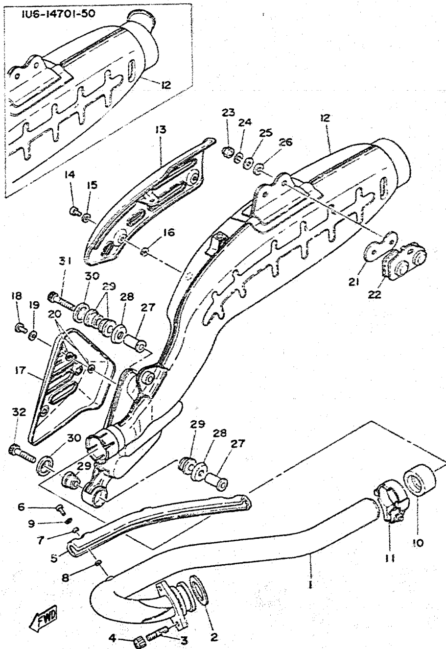
Fig. 17 EXHAUST
