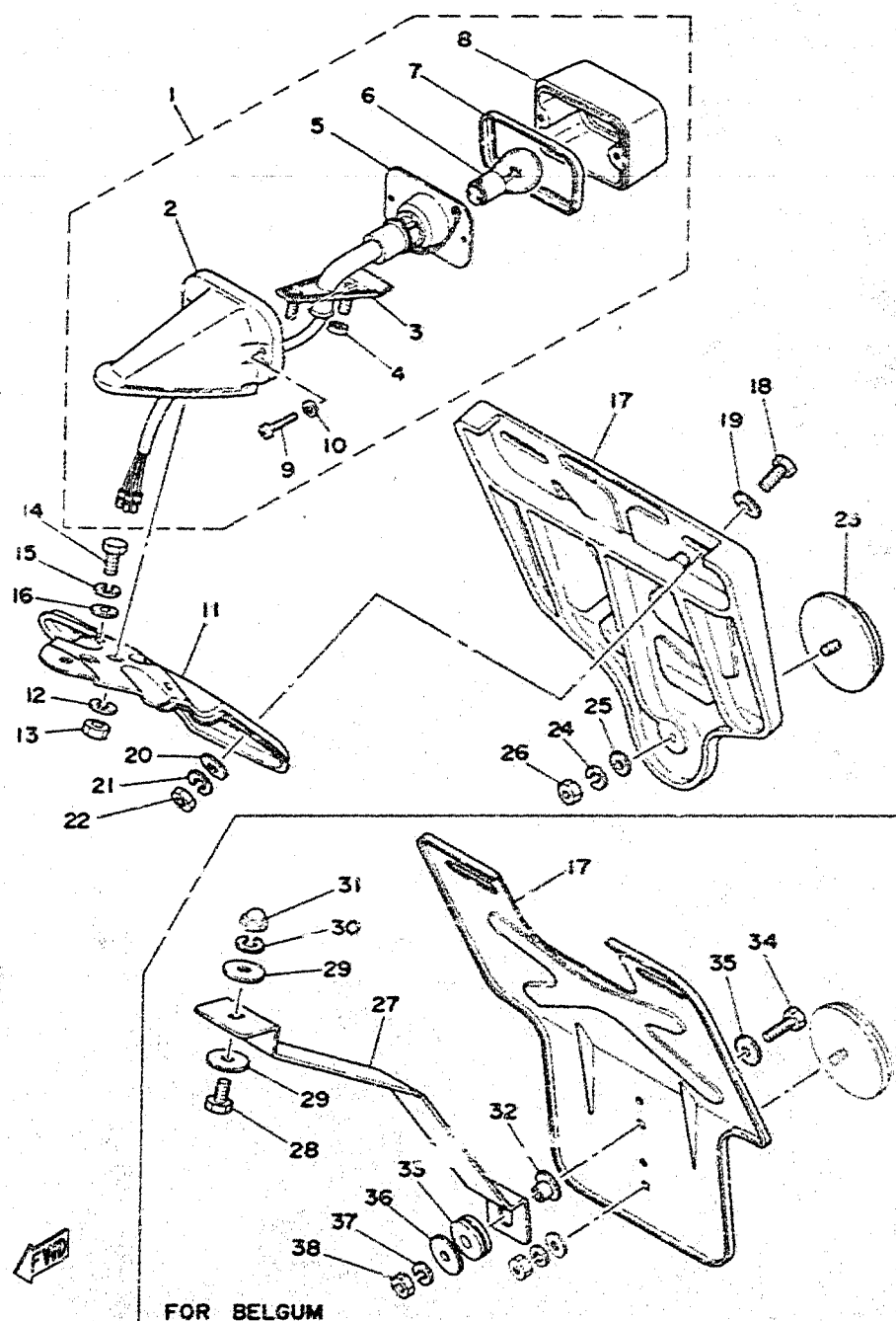
Fig. 38 TAIL LAMP 4
