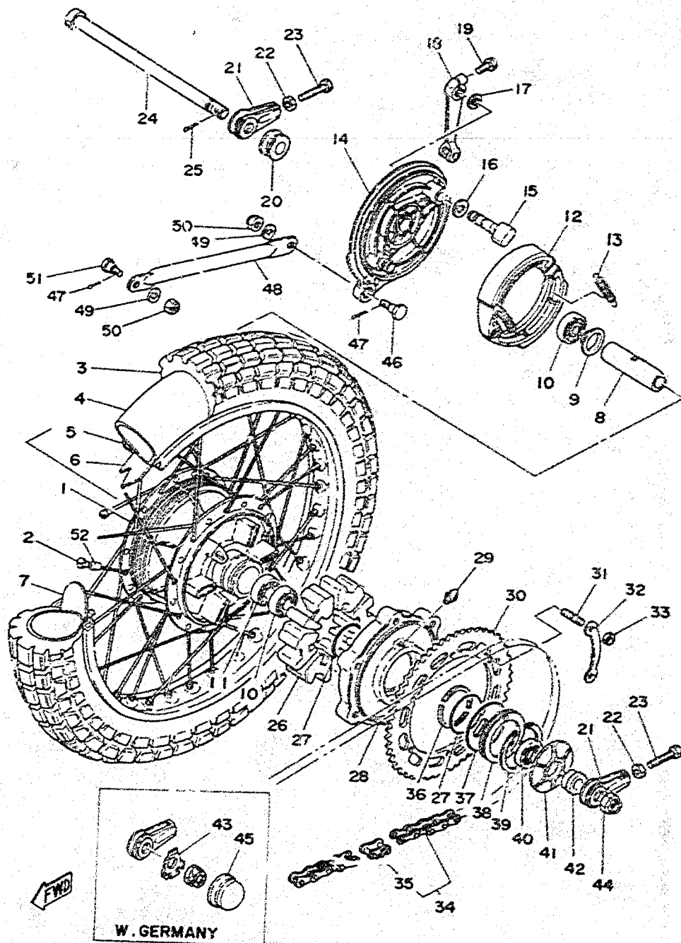
Fig. 30 REAR WHEEL
