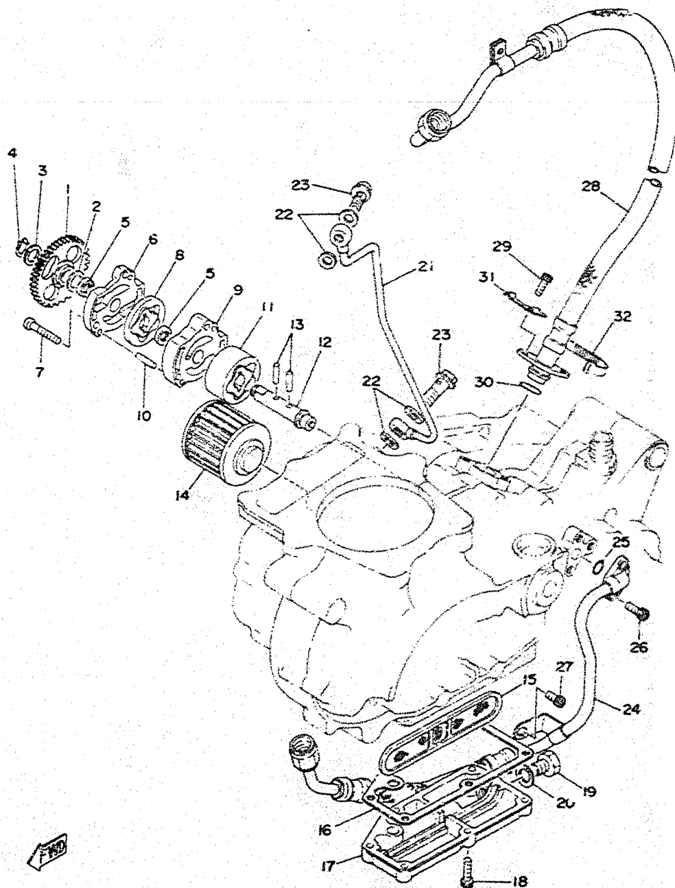
Fig. 8 OIL PUMP · OIL CLEANER
