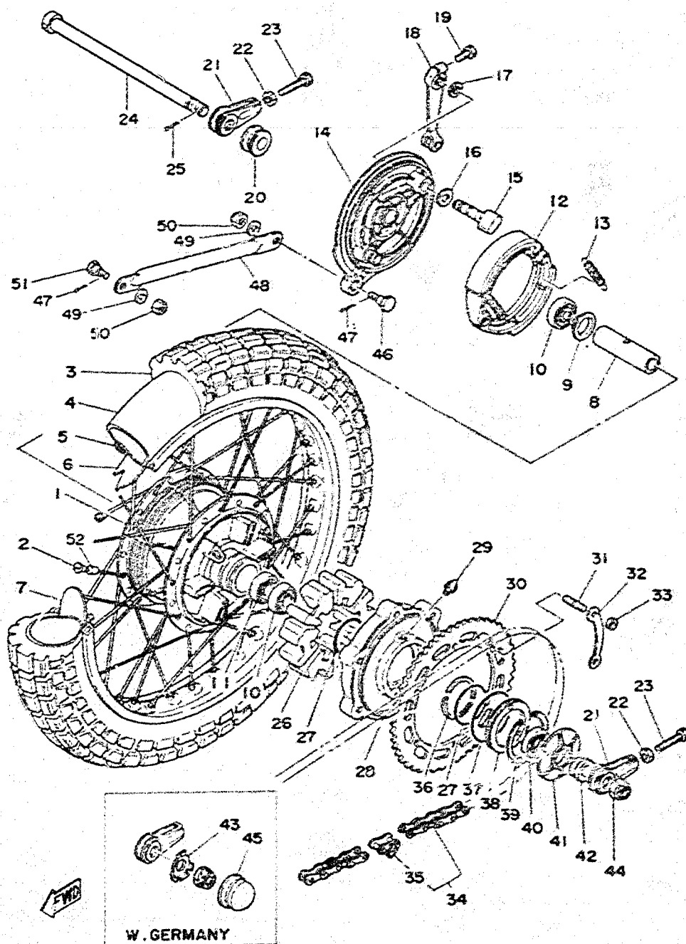
Fig. 30 REAR WHEEL
