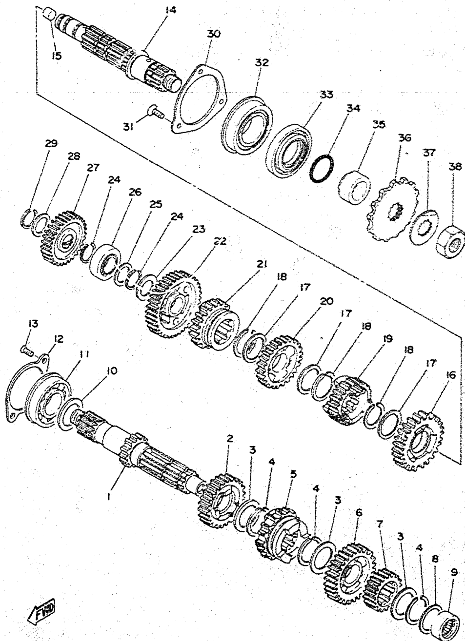
Fig. 11 TRANSMISSION
