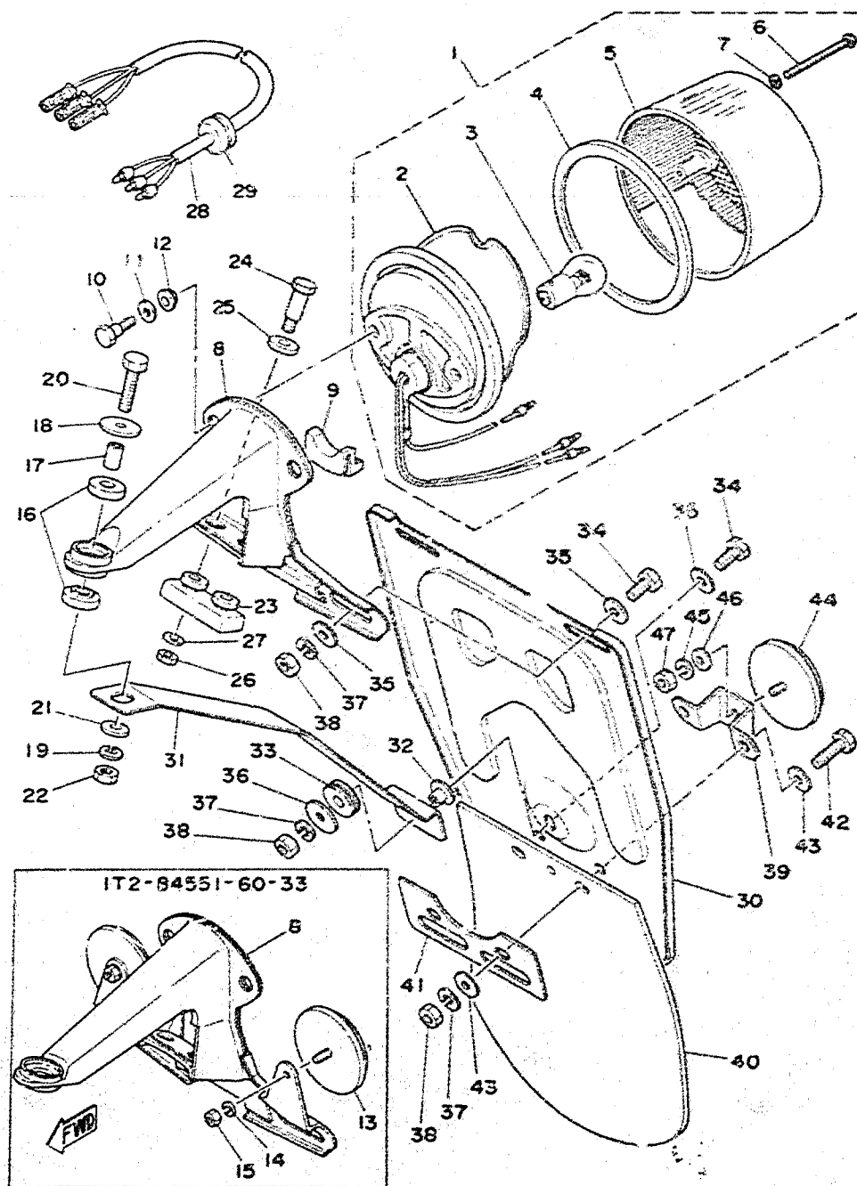
Fig. 36 TAIL LAMP 2
