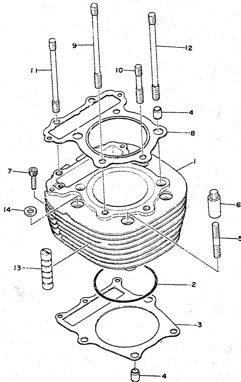
Fig. 2 CYLINDER
