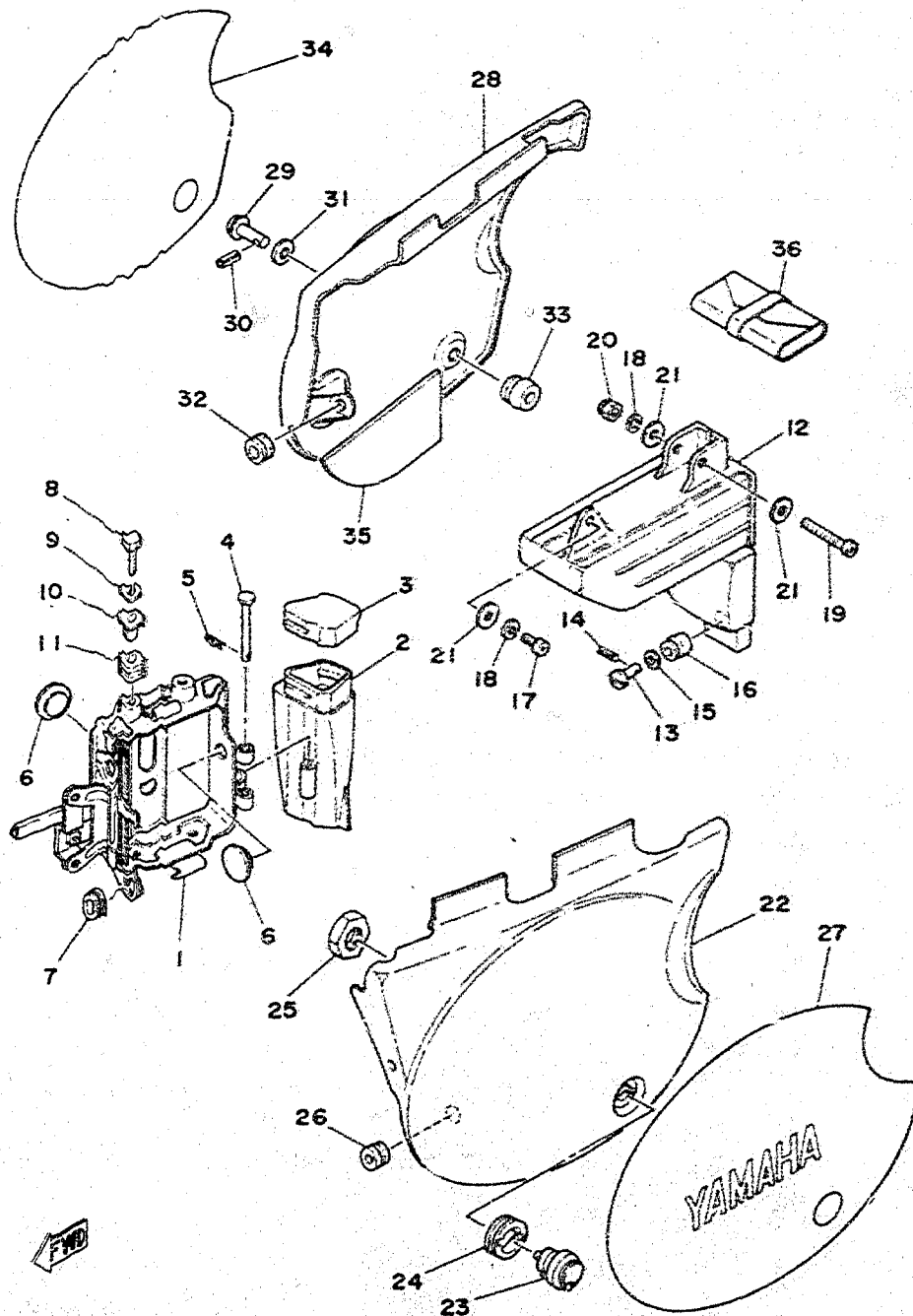
Fig. 20 SIDE COVER · BATTERY BOX
