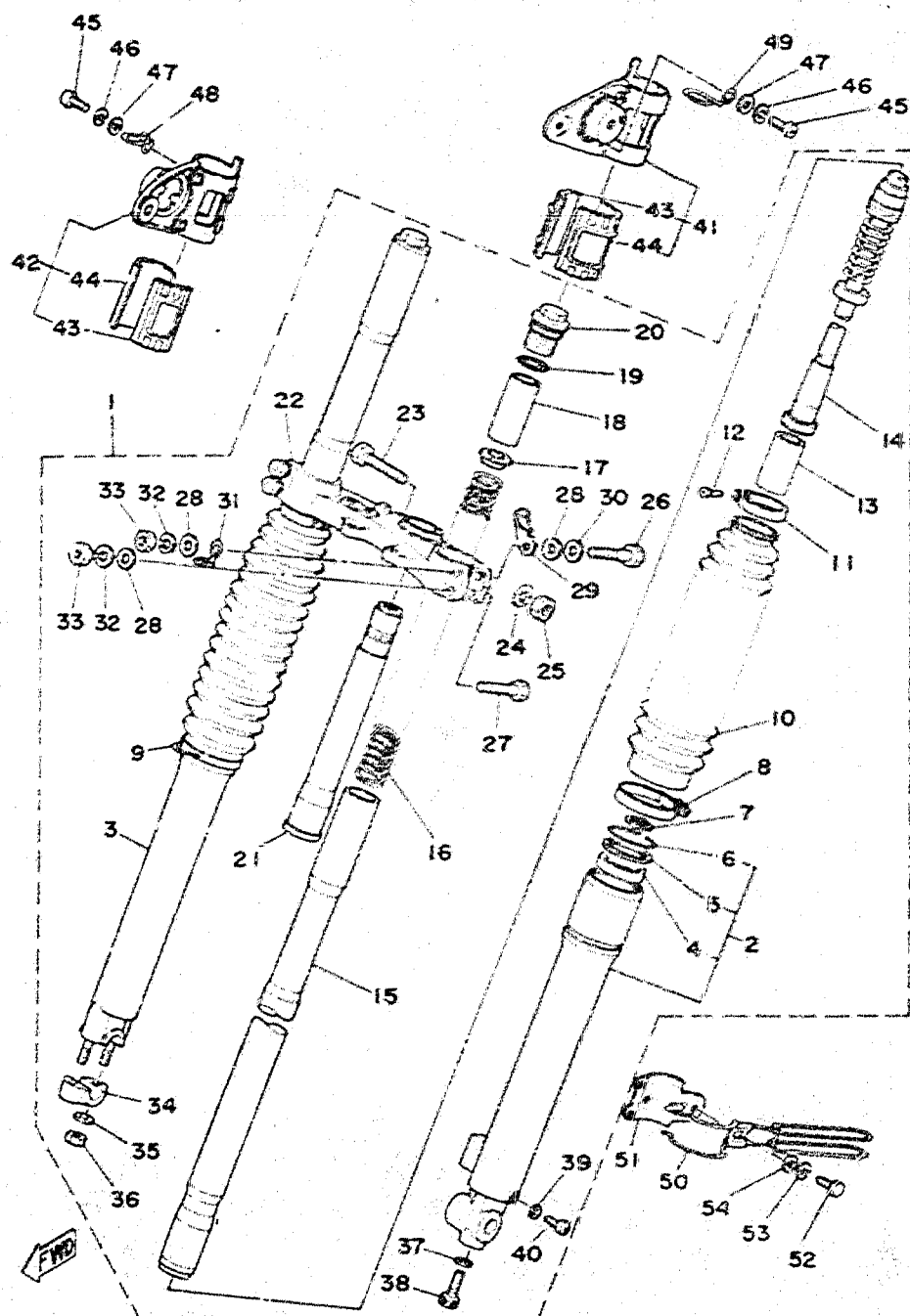
Fig. 24 FRONT FORK
