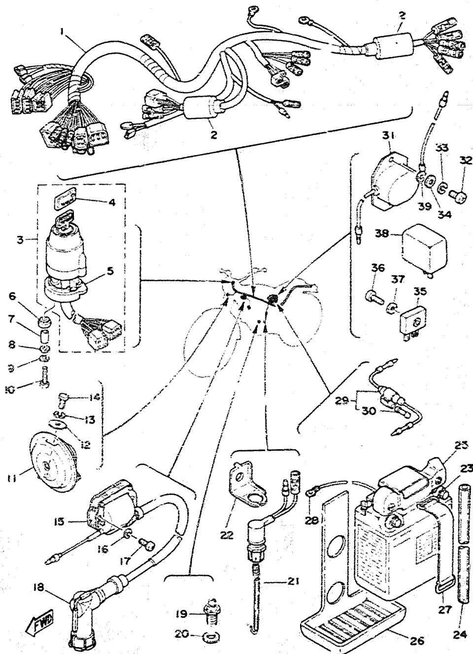
Fig. 40 ELECTRICAL
