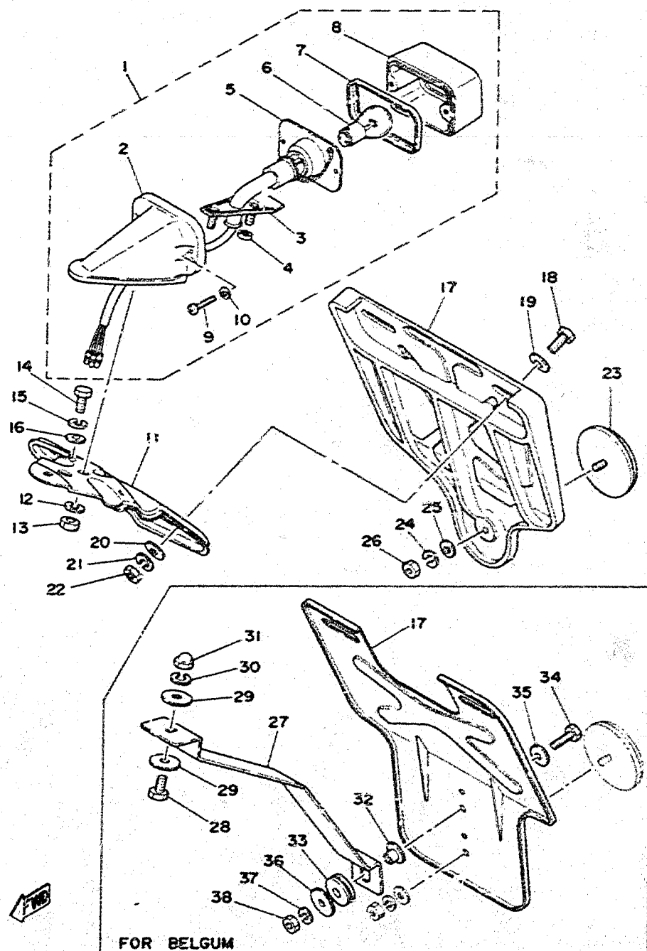
Fig. 38 TAIL LAMP 4
