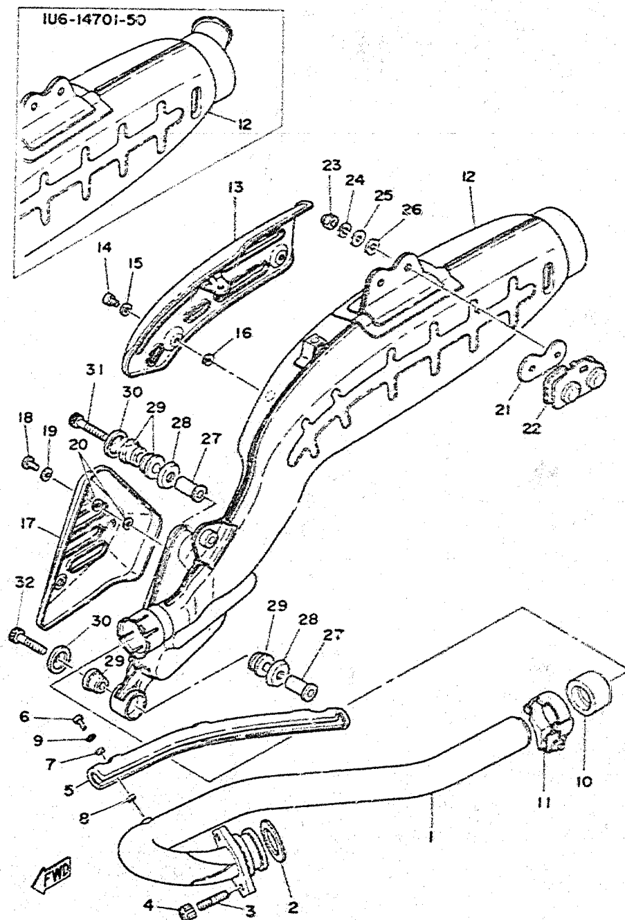
Fig. 17 EXHAUST
