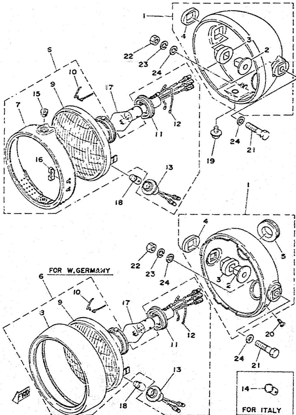
Fig. 31 HEAD LAMP 1
