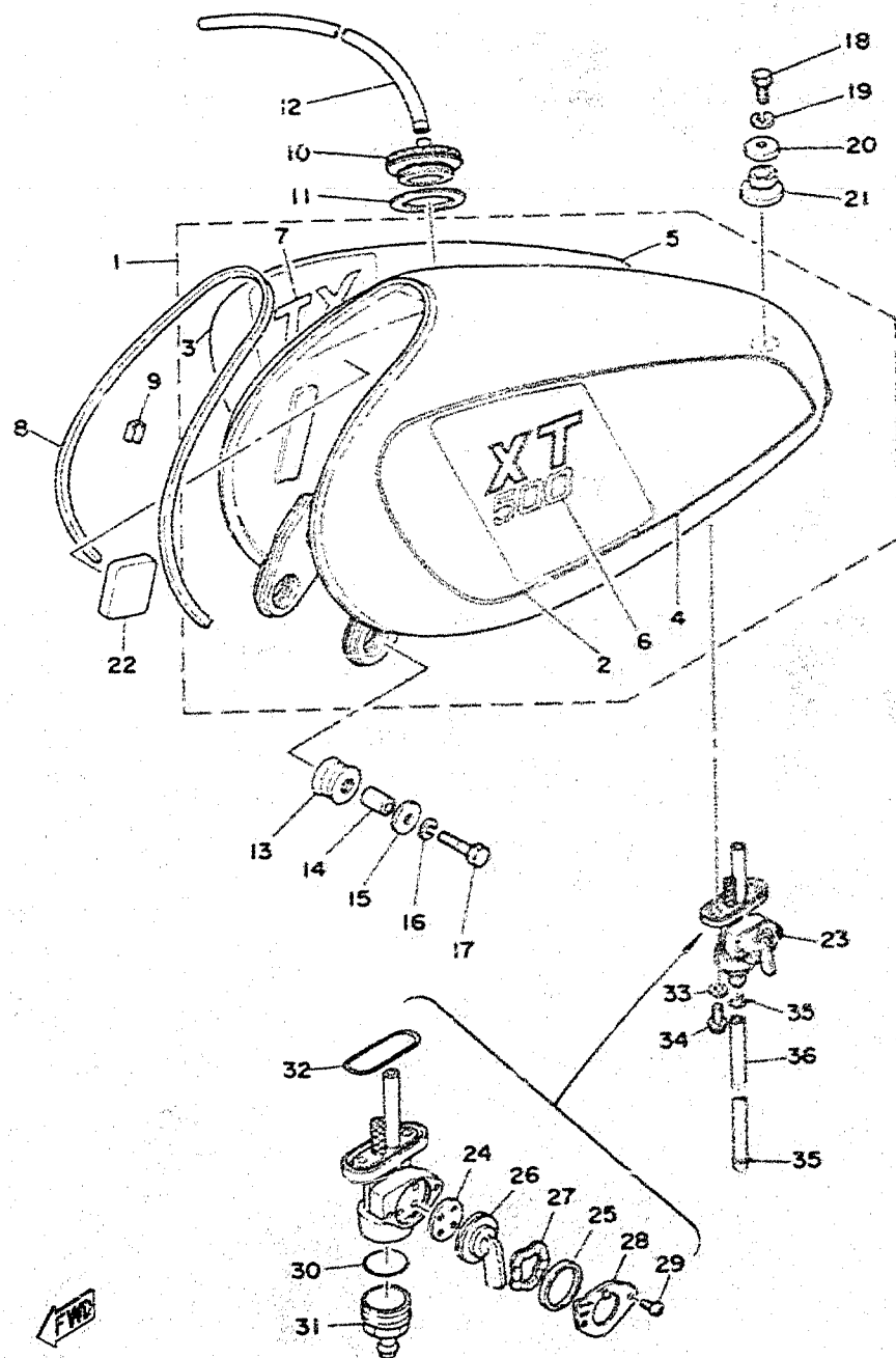
Fig. 27 FUEL TANK
