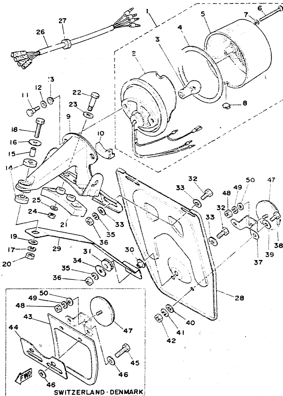
Fig. 35 TAIL LAMP 1
