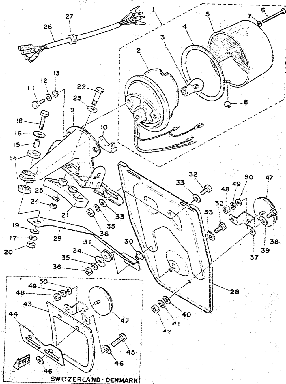
Fig. 35 TAIL LAMP 1
