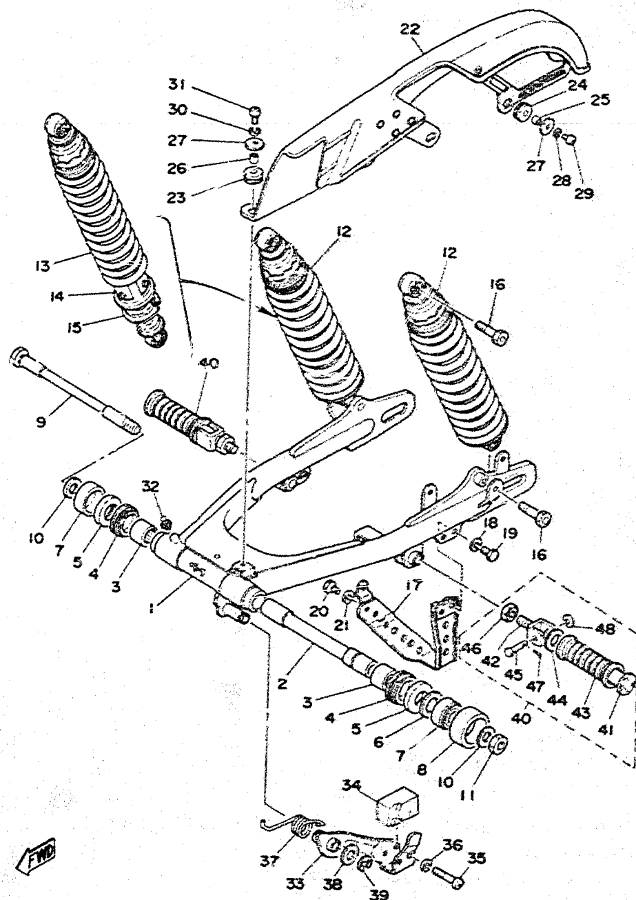
Fig. 22 REAR ARM · REAR CUSHION · CHAIN CASE
