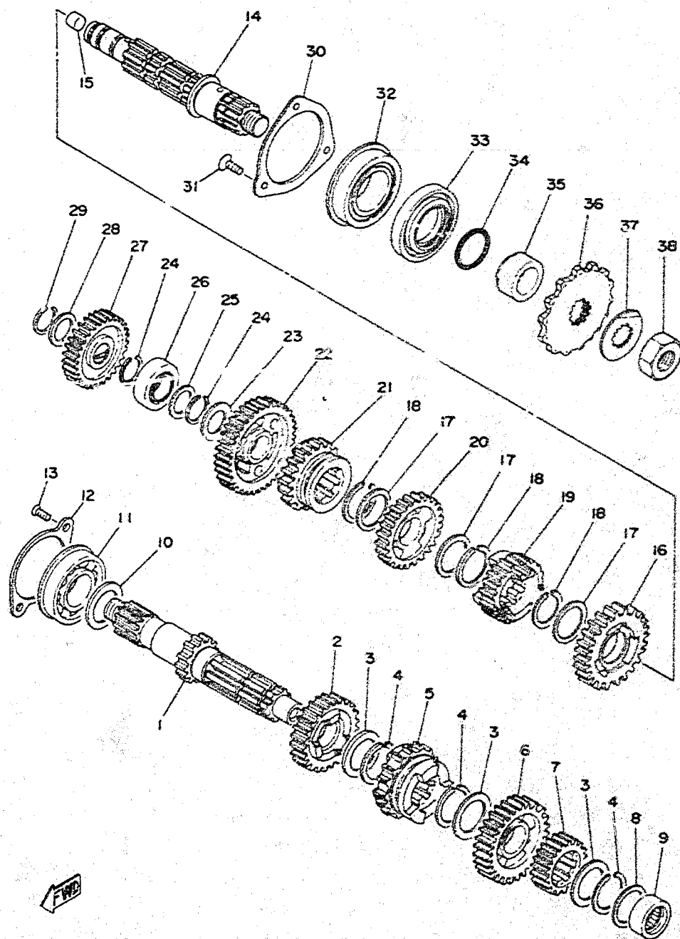
Fig. 11 TRANSMISSION
