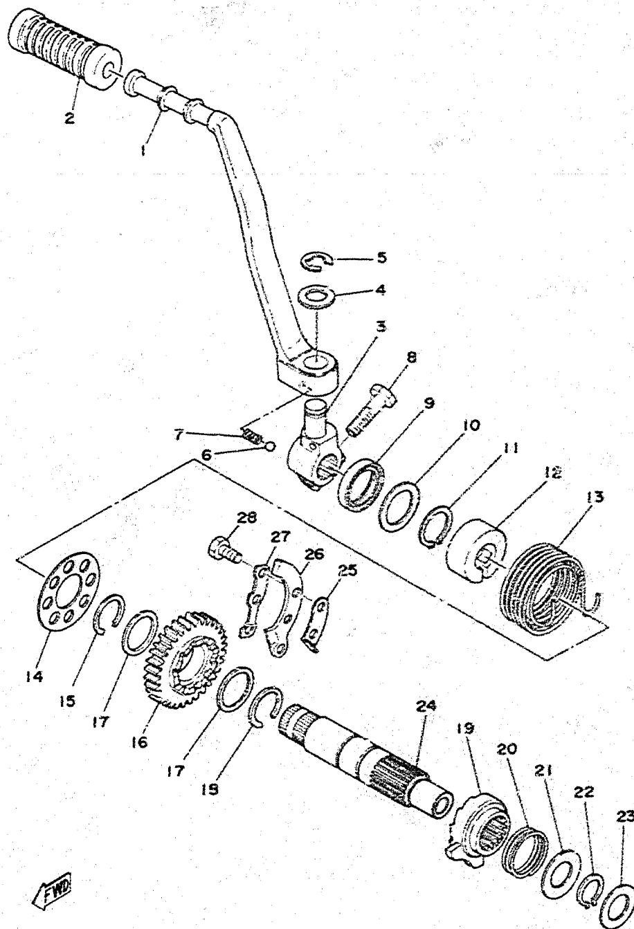
Fig. 14 KICK STARTER
