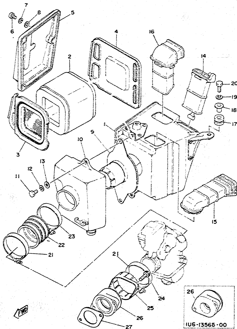
Fig. 15 INTAKE
