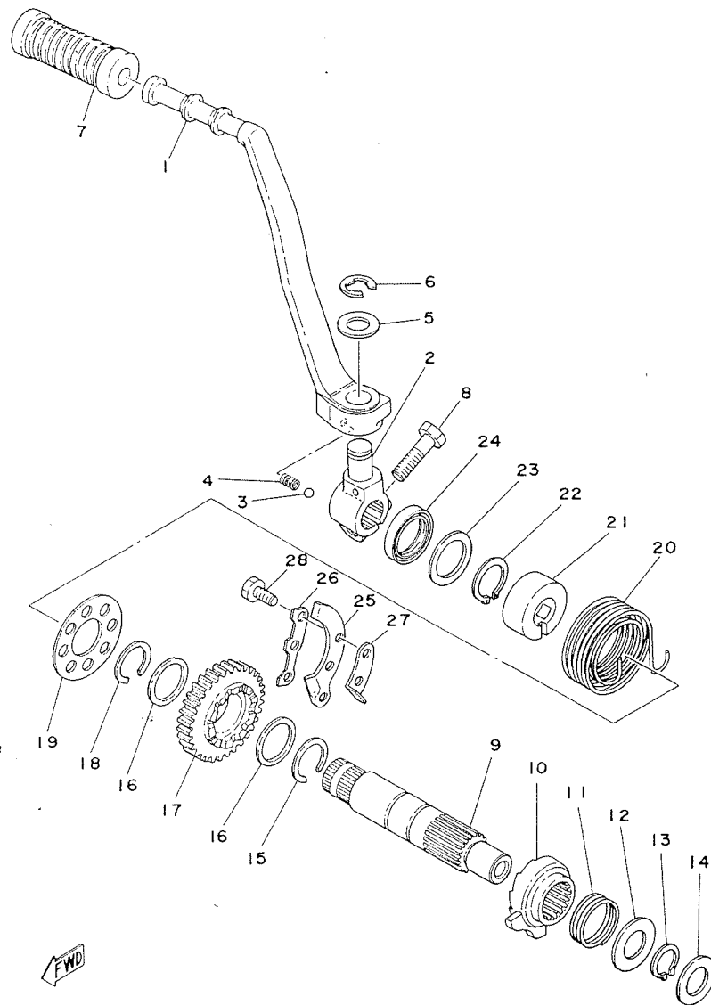
Fig. 13 KICKSTARTER
