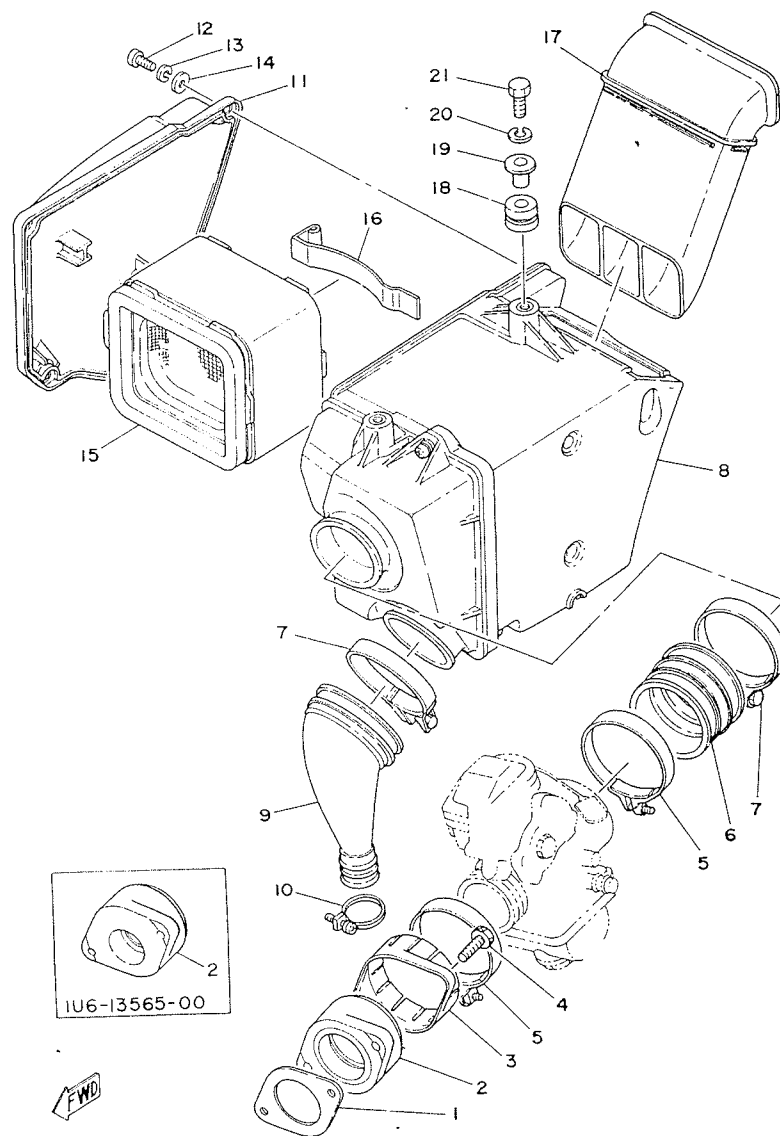
Fig. 14 ADMISSION
