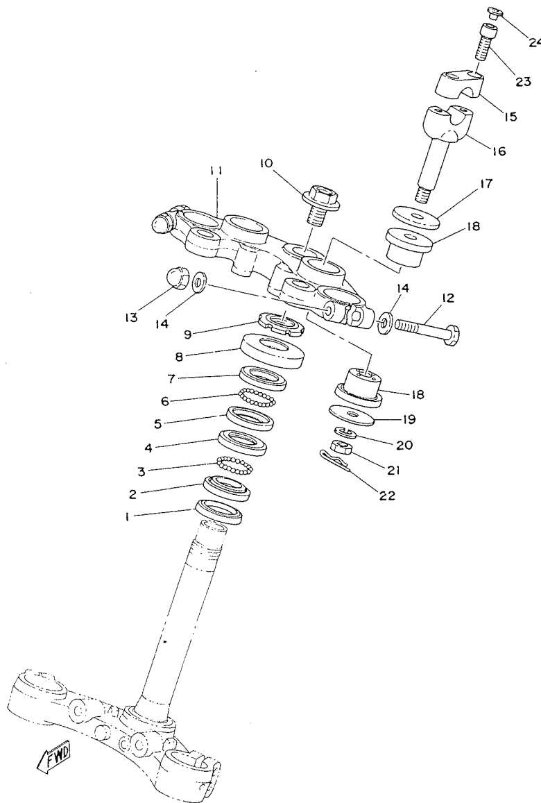
Fig. 24 DIRECTION
